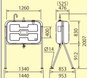
KS2-490FJ／500FJ
