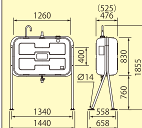
KS2-490RJ／500RJ
