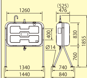
KS2-490SJ／500SJ
